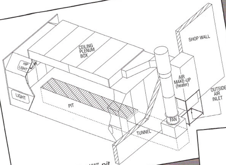
Rear vertical AMU w/"I" pit
