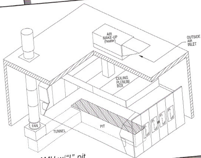
Roof mount AMU w/"L" pit
